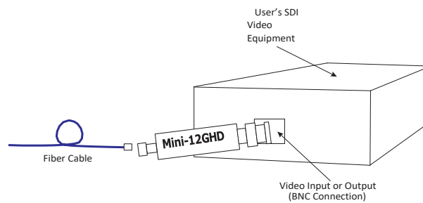
Figure 2-2 Electrical Connection
